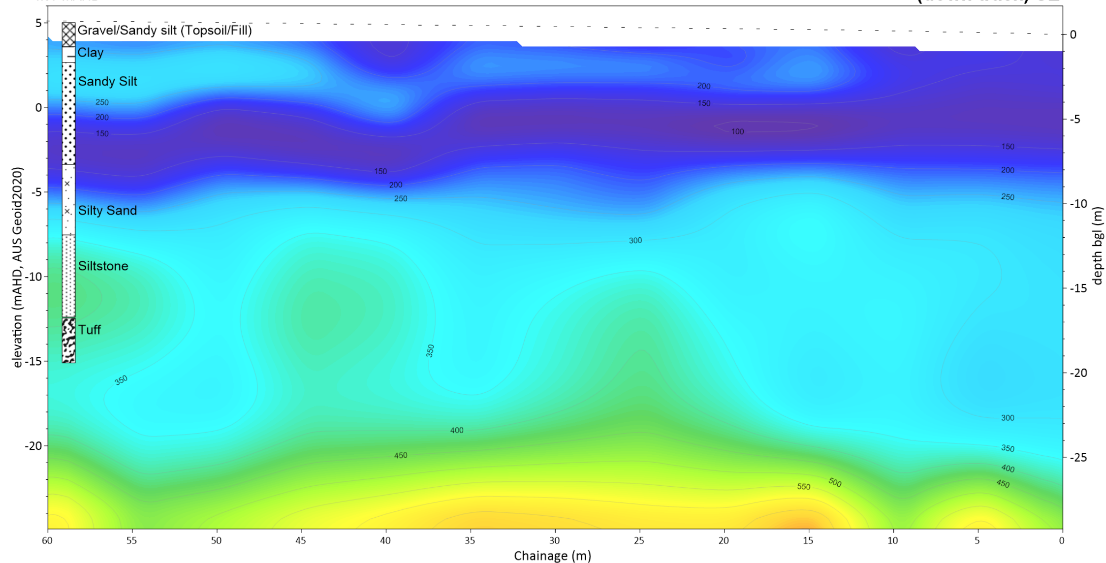
Seismic Line MASW AU-GP 145-1
